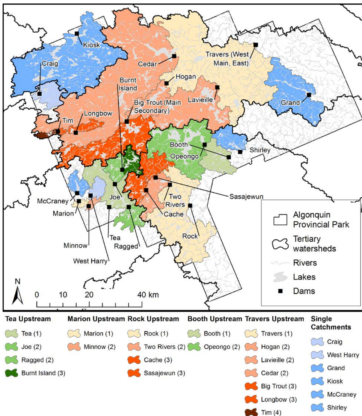
Figure 11. Upstream catchment of each dam in Algonquin Provincial Park. They range from 30 cm to a few metres tall. Dams not passable to fish protect the catchment. Some watersheds have multiple dams along the same river system, which means more isolation for areas upstream of all dams. For example, in the Madawaska watershed, Opeongo Lake is upstream of both the dam at Booth Lake and the dam on the east arm of Opeongo.
