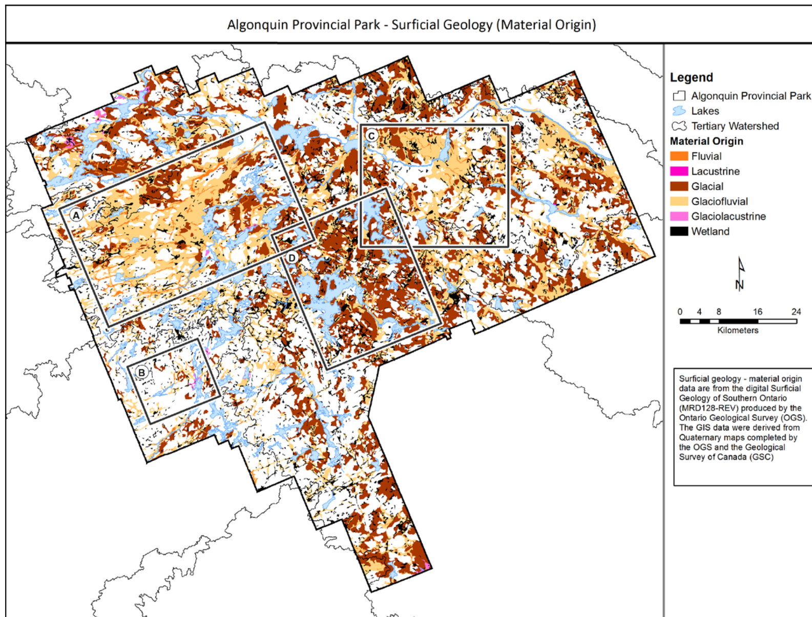
Figure 10. The distribution of material origin for surficial geology in Algonquin Park.
