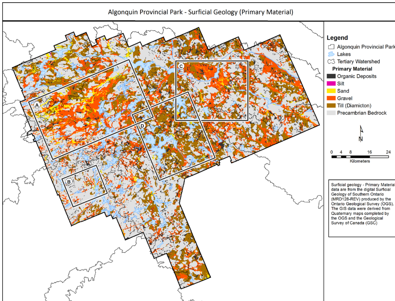
Figure 9. The distribution of primary surficial glacial material in Algonquin Park. Grey lines are tertiary watershed boundaries. Boxes A–D are specific regions of the park referred to in the text for Figures 9–11.
